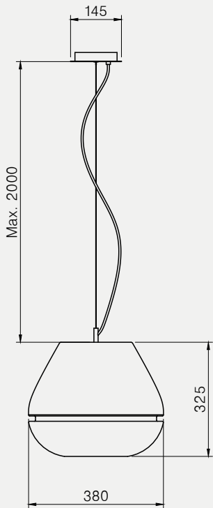
T1 IP20 E27 GLS60 led 15w 2700K 1500lm
