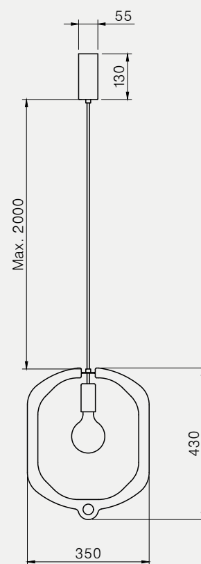
JEWEL 45 IP20 E27 G125 led bulb 5w opal 2500K 550lm
