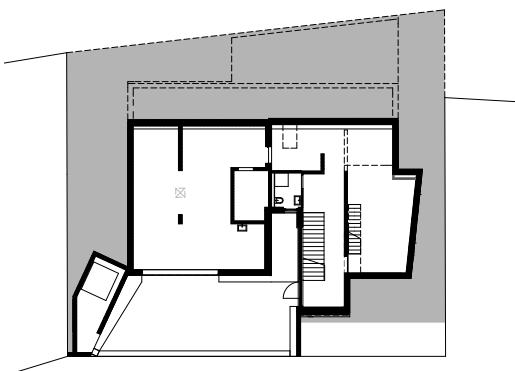
BASEMENT FLOOR 1:500
