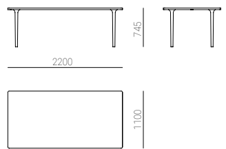
Rectangular 220 x 110
