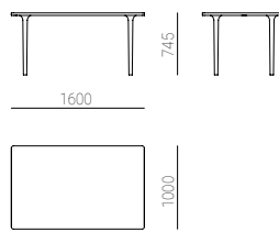
Rectangular 160 x 100
